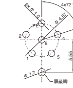
6Pin
